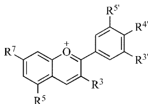
Figure 1. The flavylium chromophore ( 1 : R^3 = R^5 = R^7 = R^{3'} = R^{4'} = R^{5'} = H ), the two flavylium-derived families of pigments (anthocyanidin 2 : R^3 = OH and 3-deoxyanthocyanidin 3 : R^3 = H ) and the most common 3-deoxyanthocyanidin patterns: apigeninidin ( 4 : R^3 = R^{3'} = R^{5'} = H and R^5 = R^7 = R^{4'} = OH ), luteolinidin ( 5 : R^3 = R^{5'} = H and R^5 = R^7 = R^{3'} = R^{4'} = OH ) and tricetanidin ( 6 : R^3 = H and R^5 = R^7 = R^{3'} = R^{4'} = R^{5'} = OH ).
