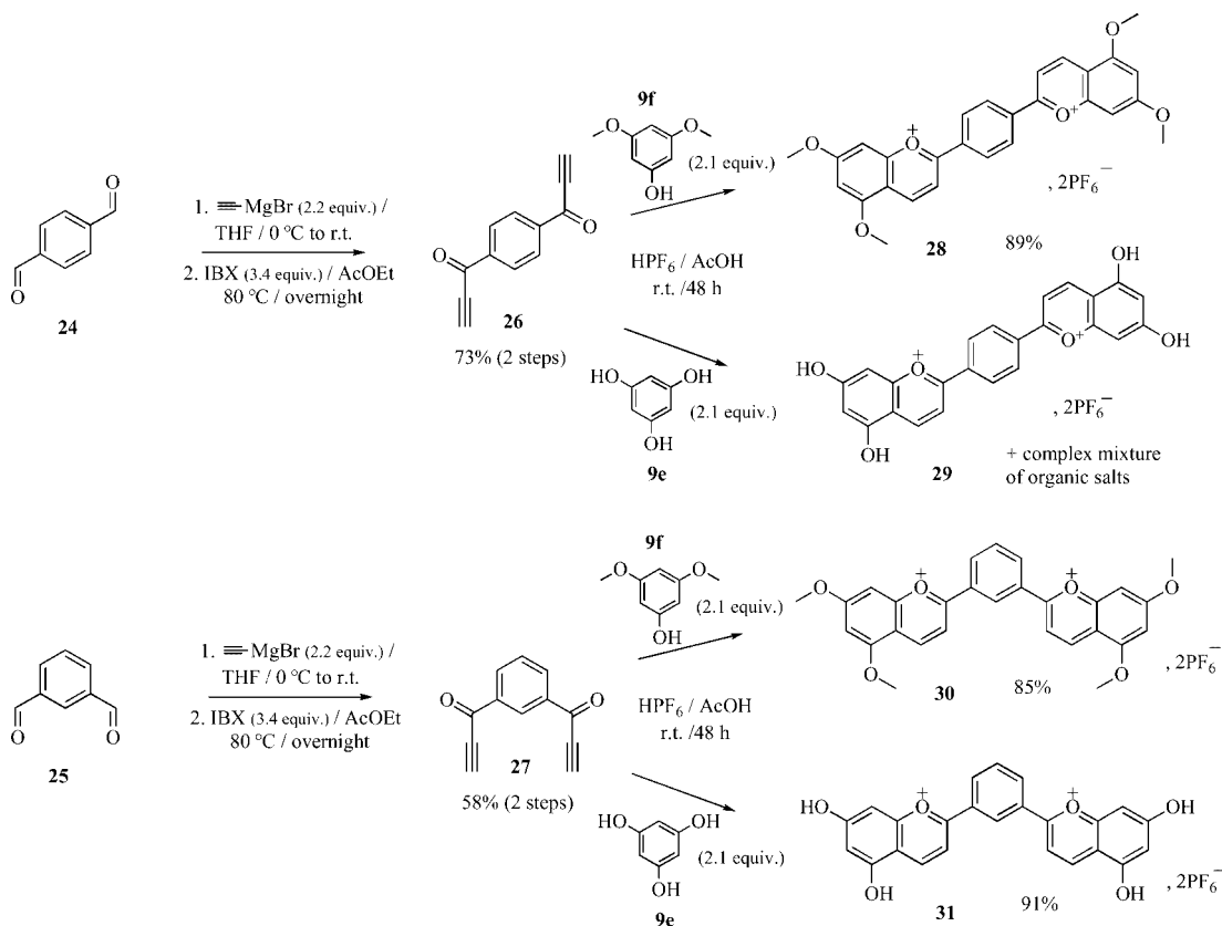
Scheme 4. Synthesis of dicationic flavylum-benzopyrylium derivatives.
