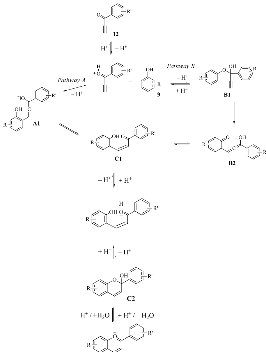
Scheme 3. Plausible mechanistic pathways for the acid-mediated condensation between an aryl ethynyl ketone and a phenolic derivative.
