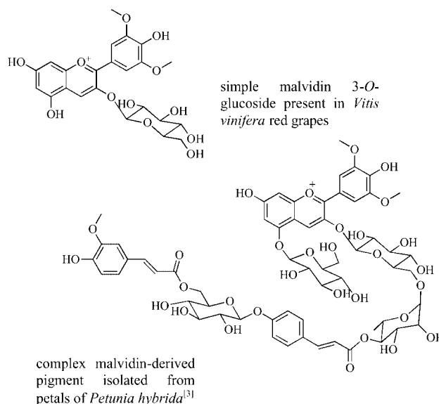
Figure 2. Illustration of the exceptional diversity existing around the flavylium nucleus with two characteristic malvidin-derived pigments.
