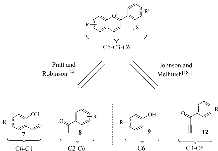
Scheme 1. Reported retrosynthetic analyses of the 3-deoxyanthocyanidin skeleton.
