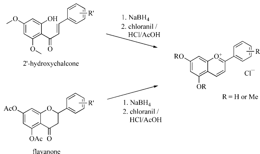
Scheme 2. Synthetic routes to 3-deoxyanthocyanidins through the chemical modification of a flavonoid precursor. [17]
